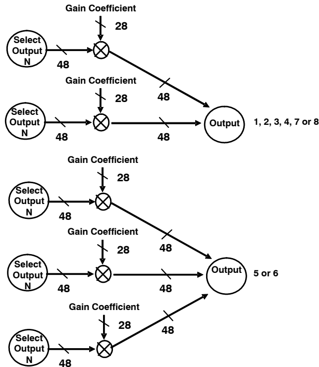
Figure 1–21. Output Mixers
