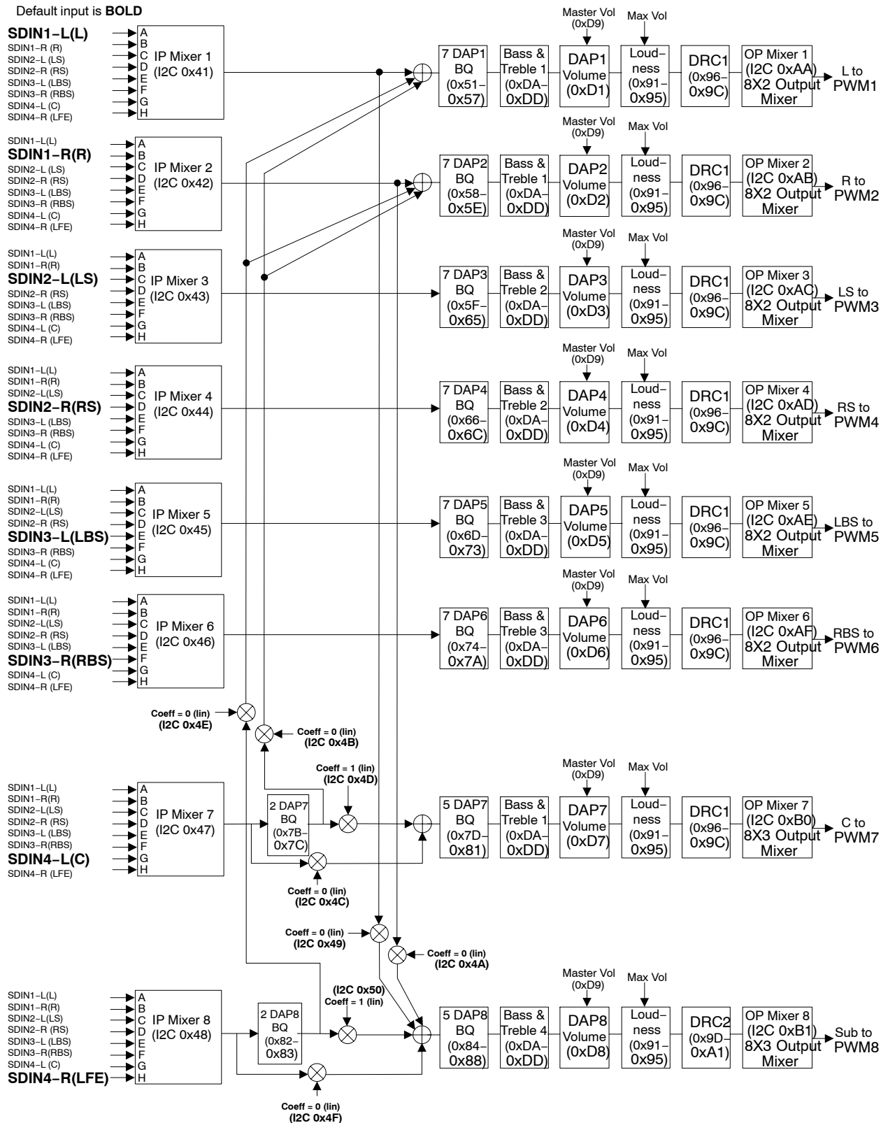
Figure 1-4. TAS5518 DAP Architecture With I 2 C Registers ( F_s \leq 96 kHz)
